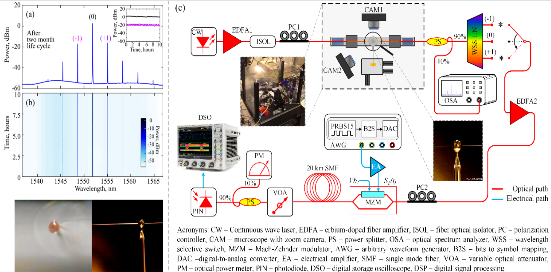
Fig. 1. Measured OFC performance over a 10-hour period: (a) optical spectrum with inset representing captured power stability, and (b) power distribution stability over the wavelength. (c) The experimental setup of the designed silica microsphere WGMR-OFC as a light source where 400 GHz spaced carriers provide NRZ-OOK modulated 2.5 and 10 Gbps data transmission over 20 km SMF fiber. Insets show tapered fiber and silica microsphere resonator positions of coupling conditions and WGMR-OFC reduced humidity and dust-prevention cover box.
