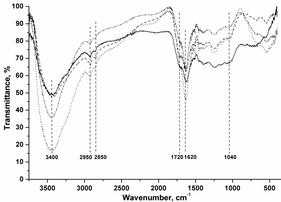
Figure 30. FT-IR spectra of peat HA from Mazais Veikeniaks Bog, at a range of depths:
