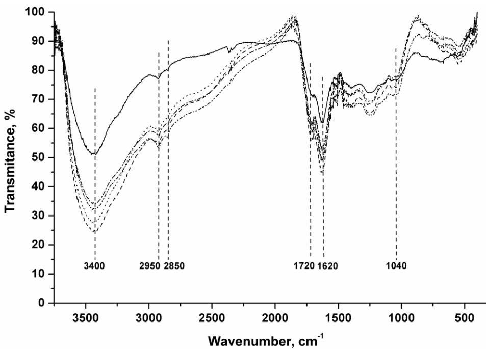
Figure 28. FT-IR spectra of peat HA from Ploce Bog, at a range of depths: — 0–30 cm - - - 31–60 cm ..... 61–85 cm - · - · - 85–110 cm - - - - 111–130 cm
