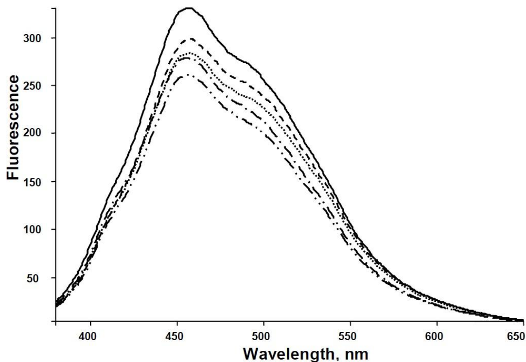
Figure 26. Fluorescence spectra of peat HA from Dižais Veikenijs Bog, at a range of depths:
