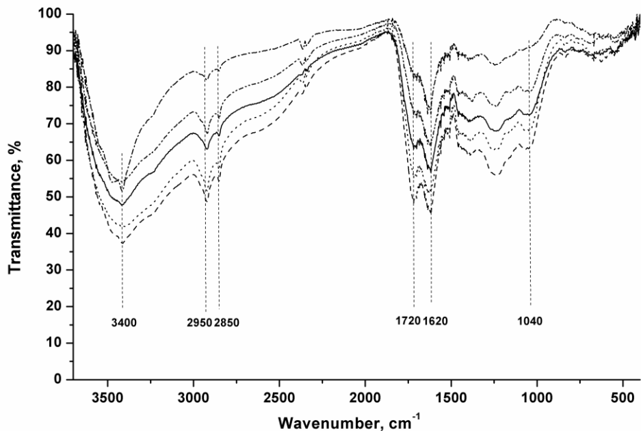
Figure 27. FT-IR spectra of peat HA from Dižais Veikenijs Bog, at a range of depths: — 0–25 cm - - - 26–52 cm ..... 53–75 cm - · - · - 76–98 cm - - - - 99–118 cm
